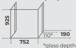
Dimensions (mm)
